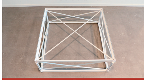
7. Place the frame on the ground with the backside (textile cross) facing up.
